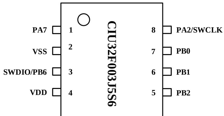
Figure 3-4 CIU32F003J5S6-SOP8 pinout
