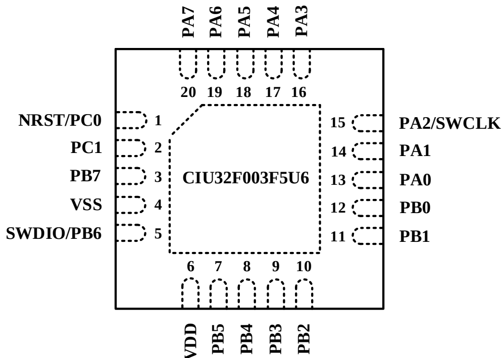
Figure 3-2 CIU32F003F5U6-QFN20 pinout
